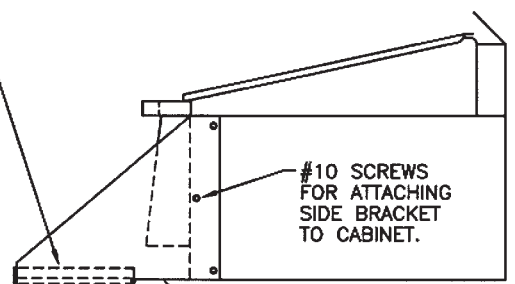
SIDE BRACKET TYP. BOTH ENDS OF GRIDDLE
